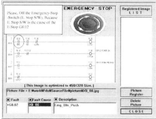
Fig. 6 FDS implemented in CNC controller
