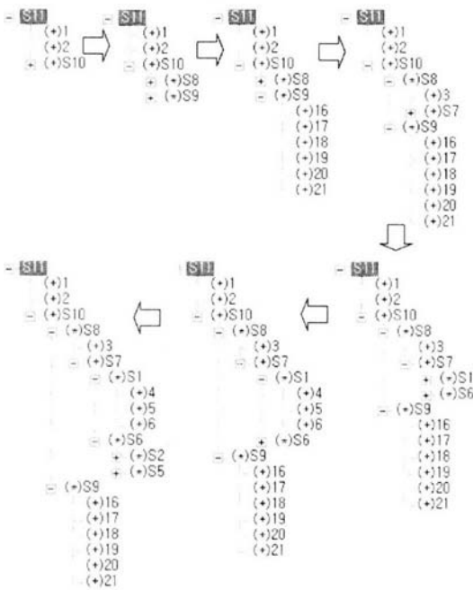
(b) SSF-tree
