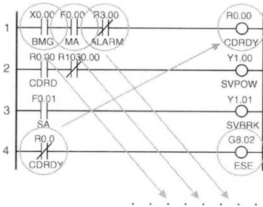
Fig. 3 PLC ladder diagram of emergency stop error (G8.02)
