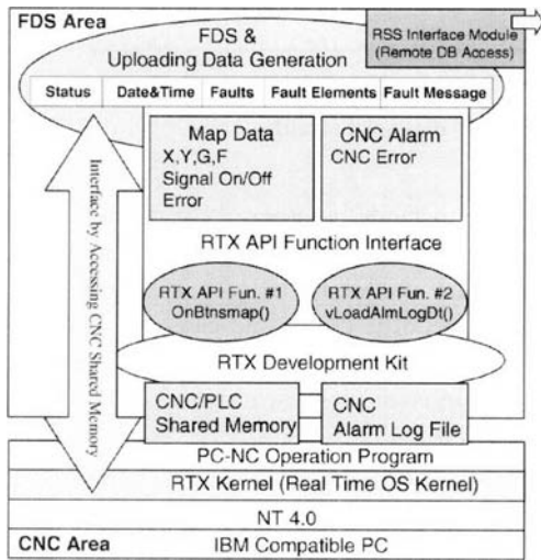
Fig. 8 Interface between FDS and CNC domain
