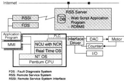
Fig. 1 Function diagram of OAC in machine-tool
