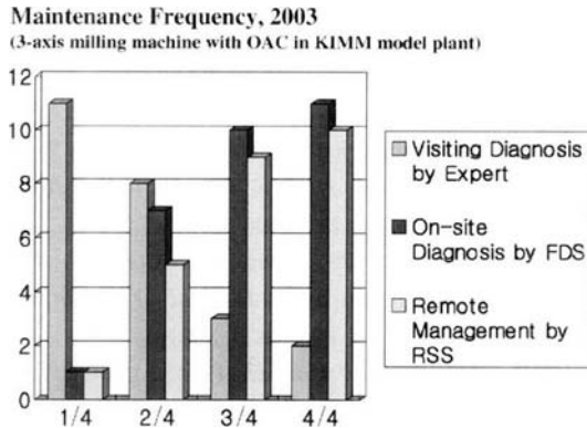
Fig. 14 Maintenance frequency of visiting and on-site
